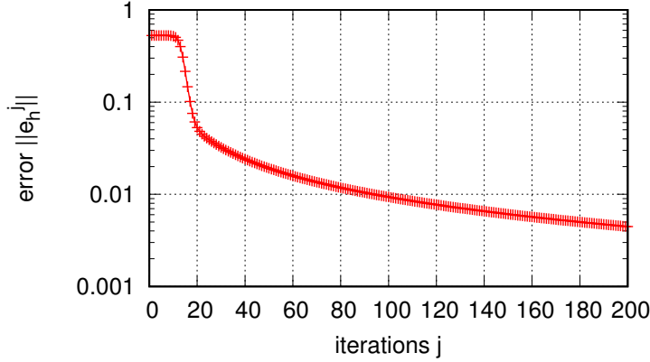
Figure 15.4: Convergence of the damped Jacobi method.
