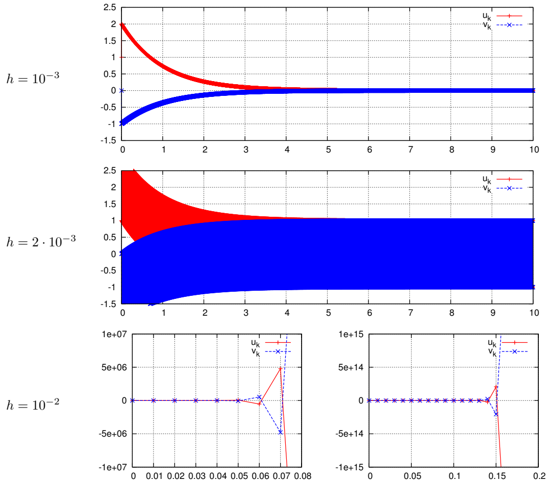
Figure 10.5: Approximate solution of (10.39) by the explicit Euler method.
